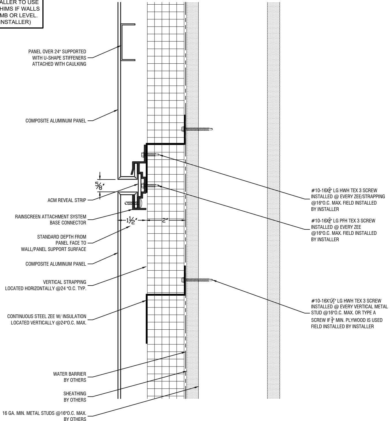
Typical Horizontal Joint Detail
