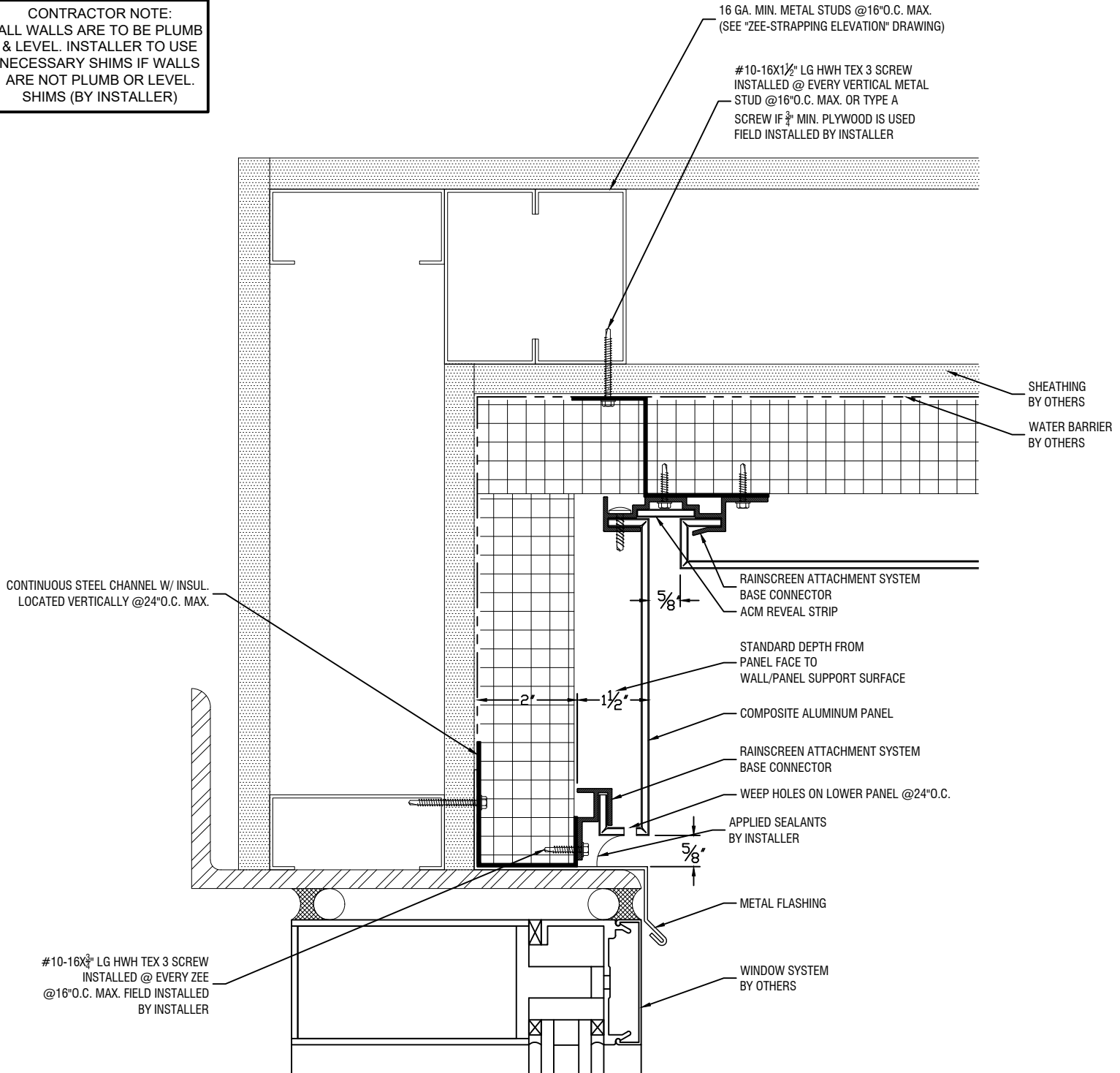
Canopy Detail
