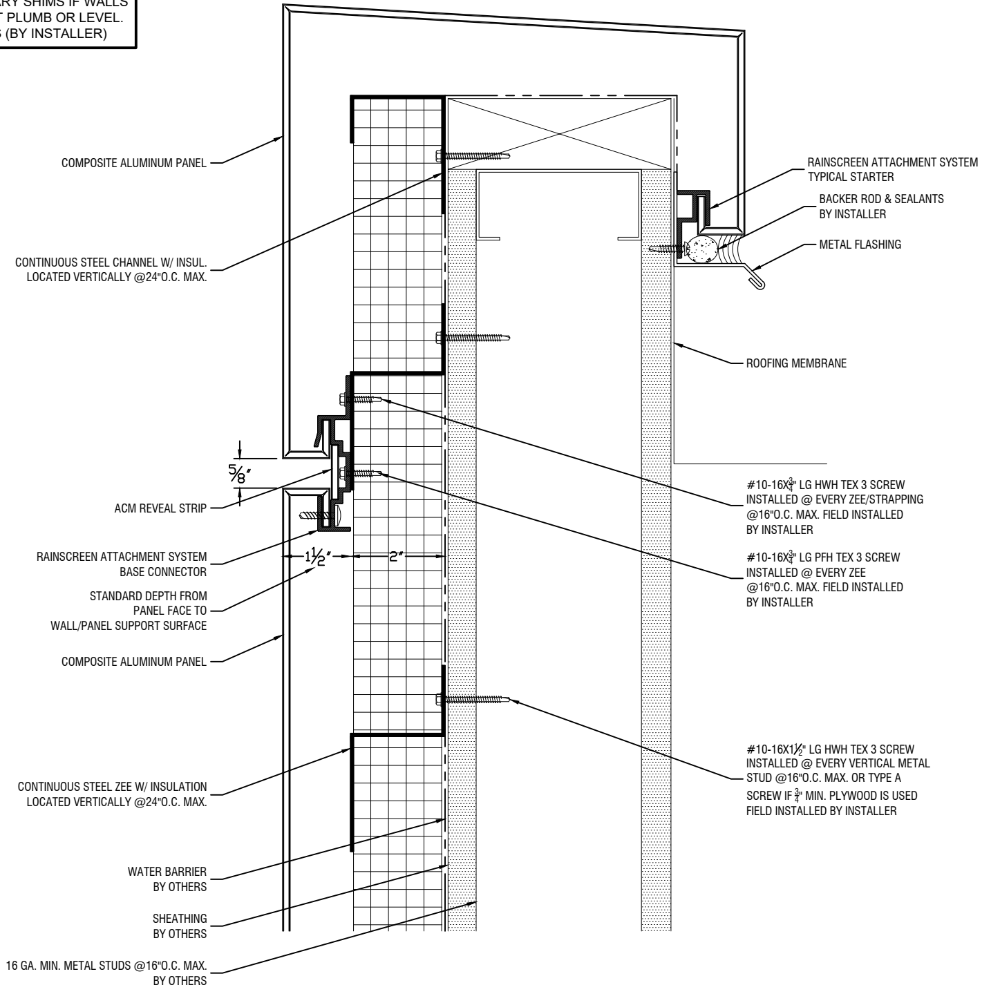
Coping Detail-2
