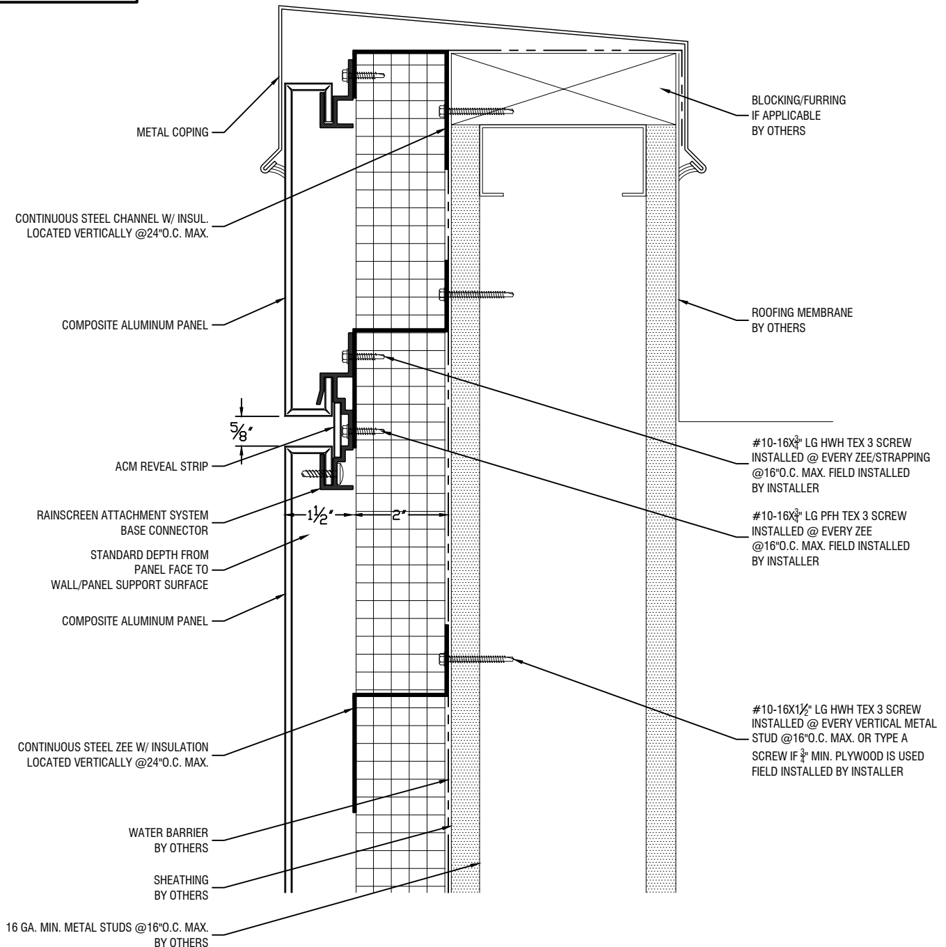
Coping Detail-1
