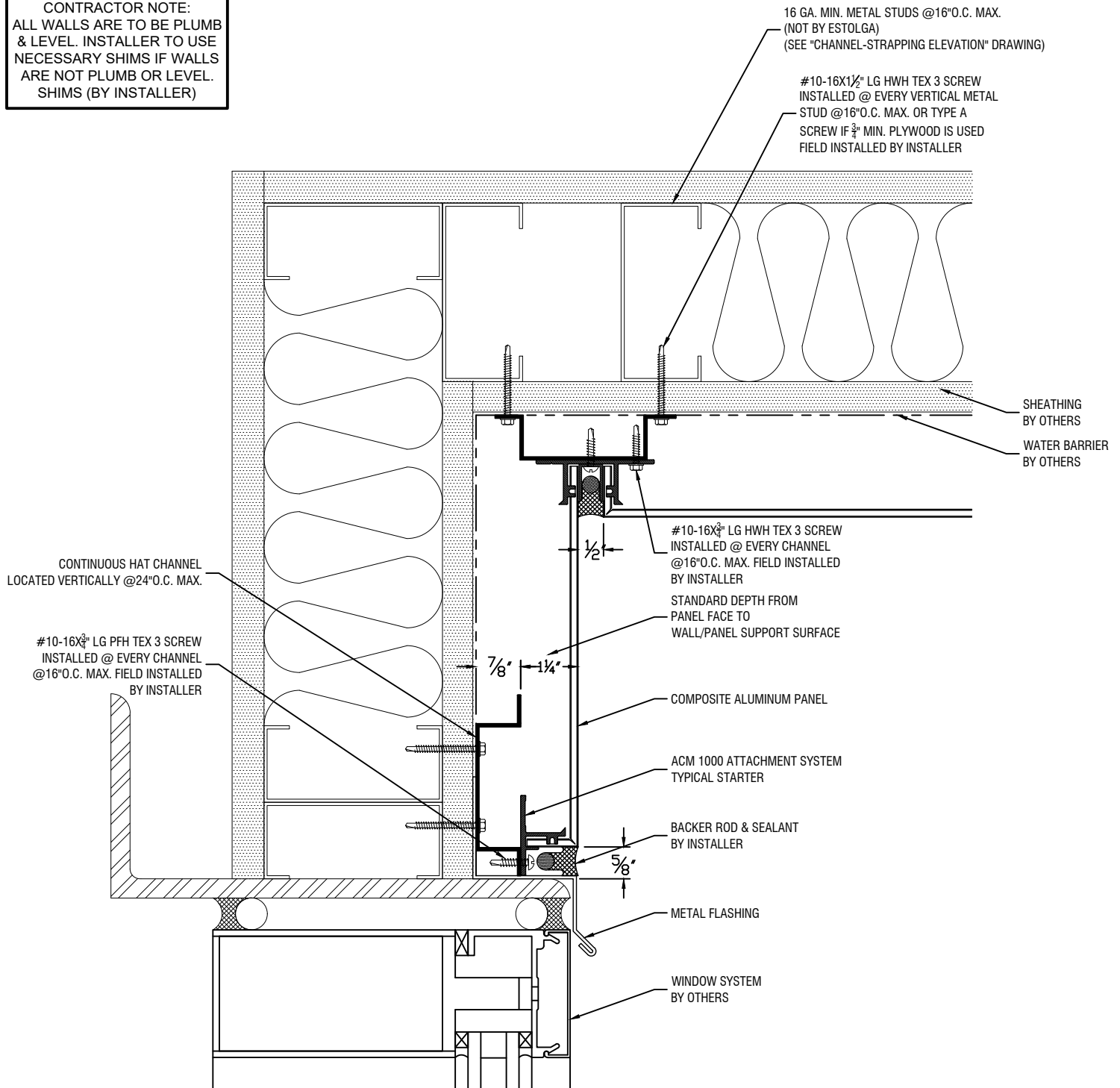
Canopy Detail
