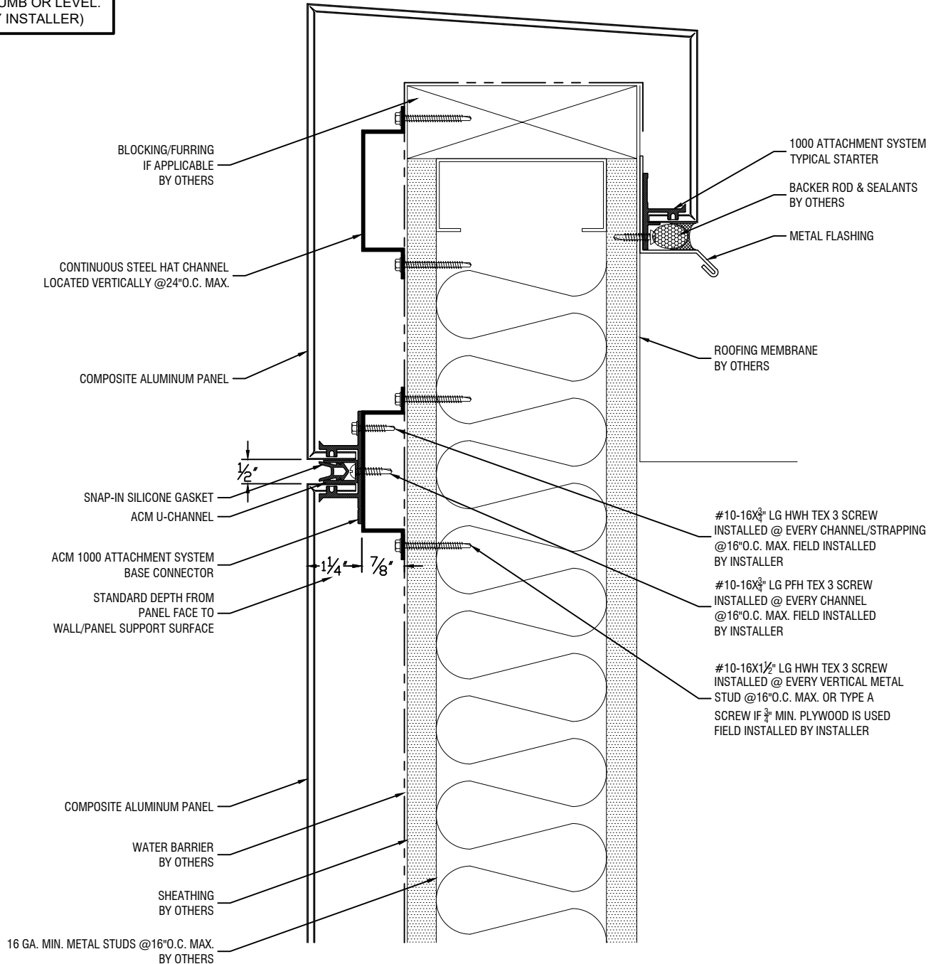
Coping Detail-2
