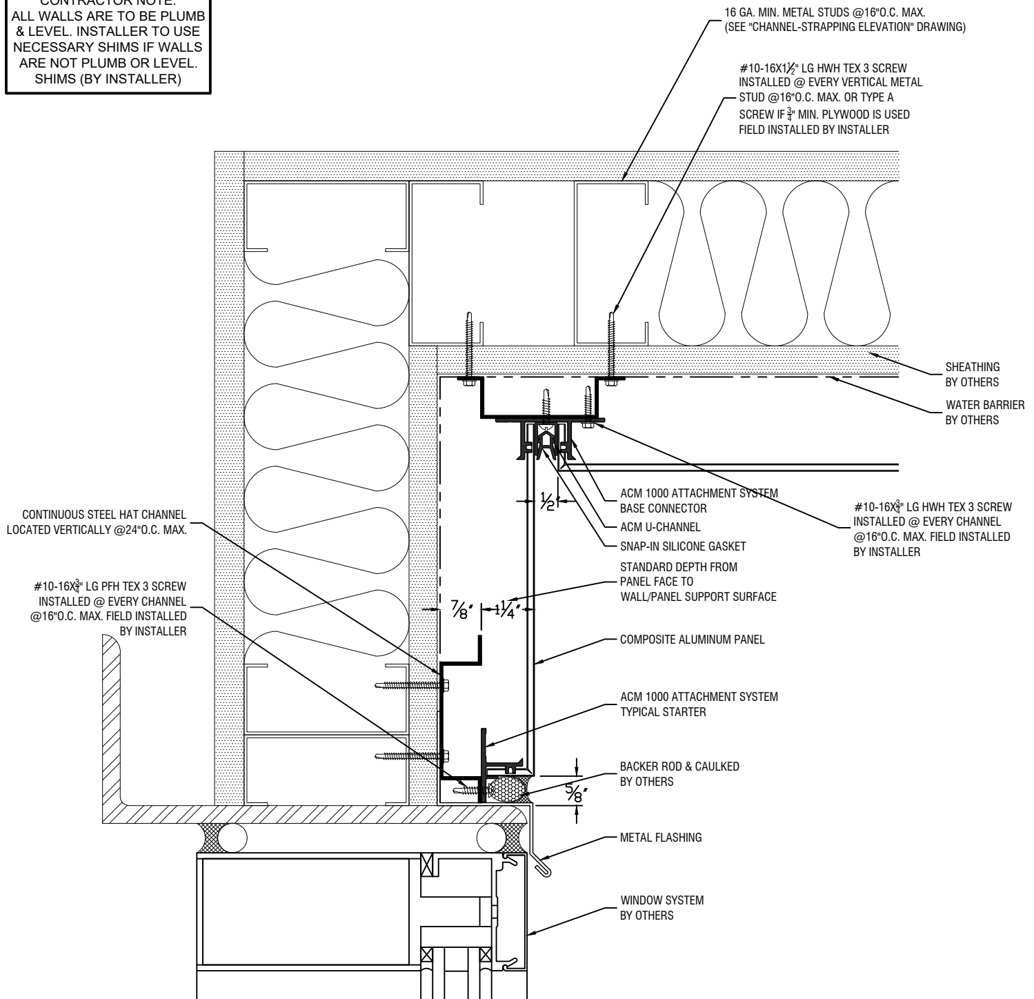
Canopy Detail
